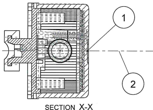
SECTION X-X
