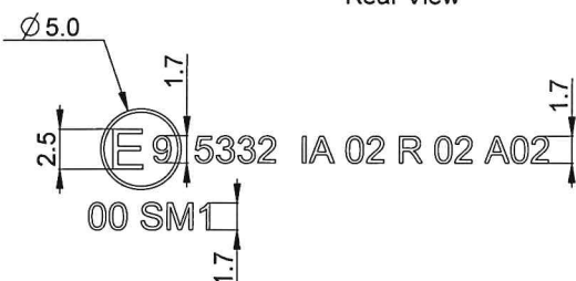
Detail A (2:1)
