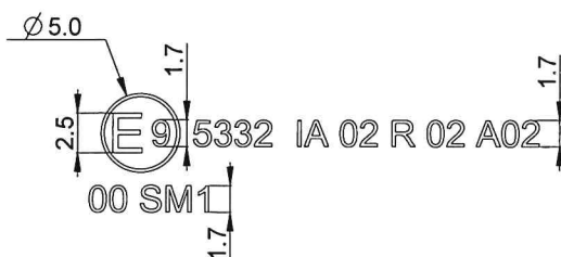
Detail A (2:1)
