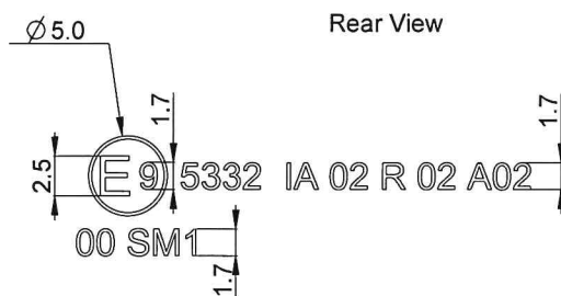
Detail A (2:1)
