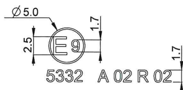
Detail A (2:1)
