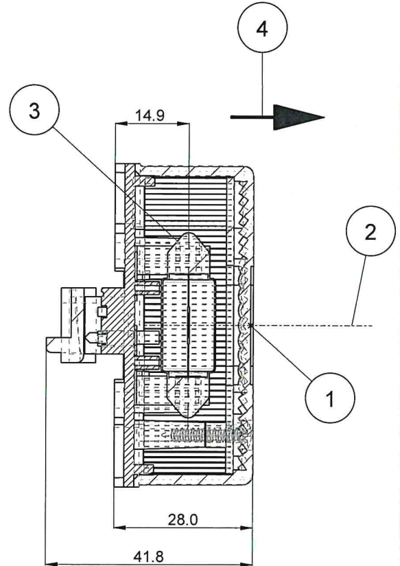
SECTION Y-Y
