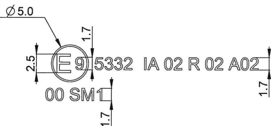
Detail A (2:1)
